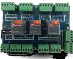
Fan Coil Multiplexing Board
