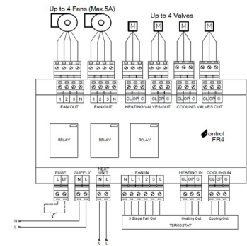
FCU Relay Box 3 Speed 220V or 24V
