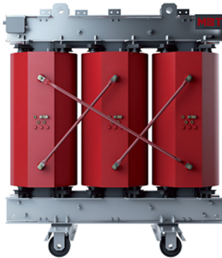
Dry Type Transformer
