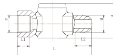
M/F type sight glass
