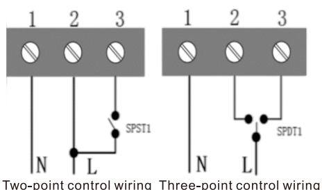
Switch output connection method, working Voltage: AC/DC 24V; AC100V...AC240V
