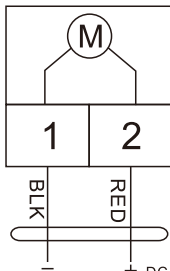
Wiring diagram: ON-OFF type
