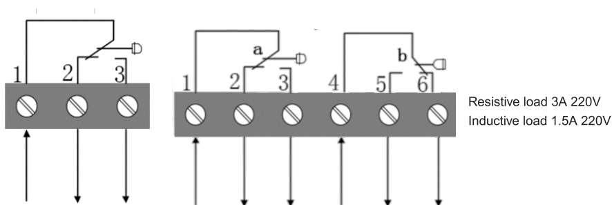
One set of auxiliary switch wiring methods Two sets of auxiliary switch wiring methods
