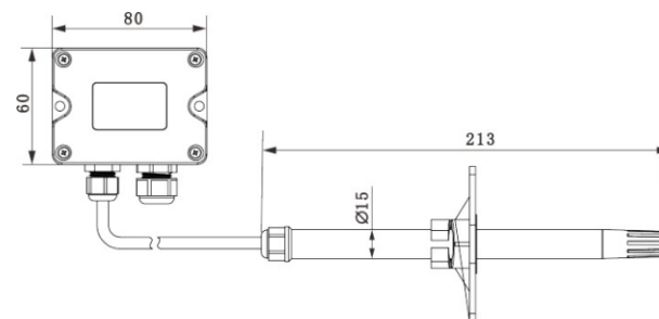
LFH10A3 Split type
