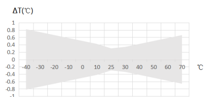
Temperature Accuracy Curve(Analog output model)
