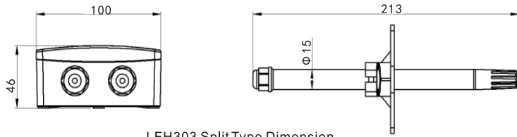
LFH303 Split Type Dimension
