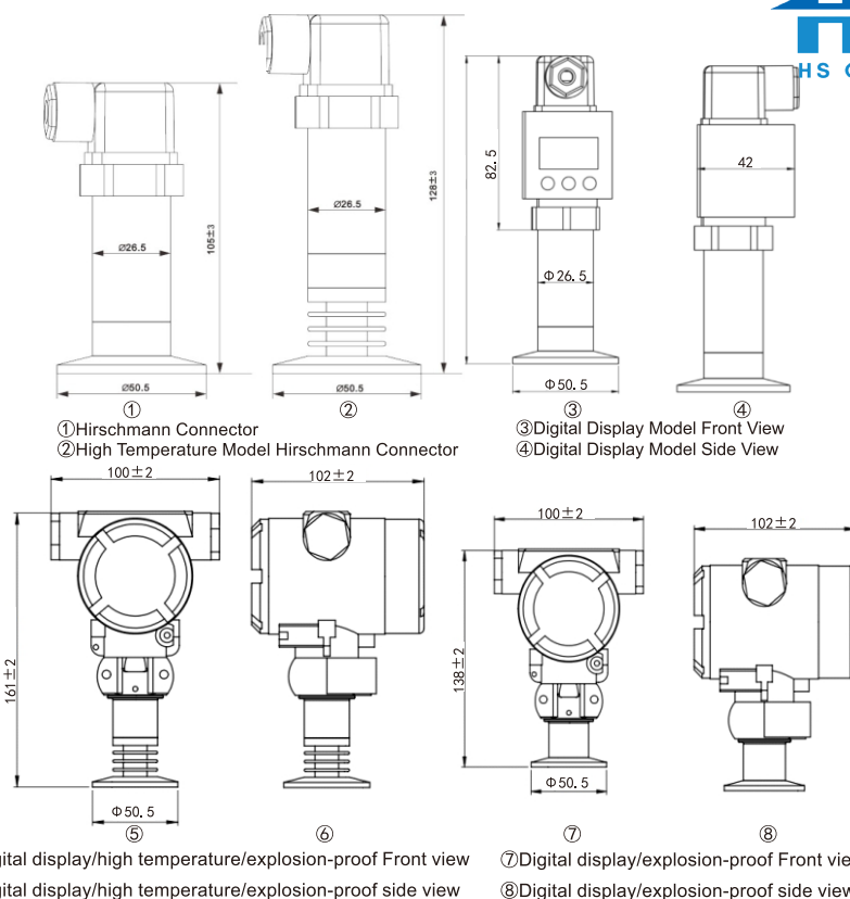
① Hirschmann Connector ② High Temperature Model Hirschmann Connector ③ Digital Display Model Front View ④ Digital Display Model Side View ⑤ Digital display/high temperature/explosion-proof Front view ⑥ Digital display/high temperature/explosion-proof side view ⑦ Digital display/explosion-proof Front view ⑧ Digital display/explosion-proof side view
