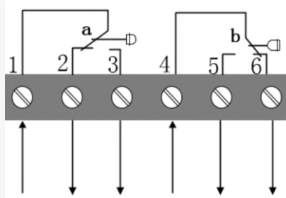
Two sets of auxiliary switch wiring methods
