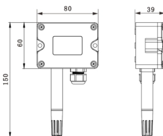
LFH10A1 Wall-mounted type
