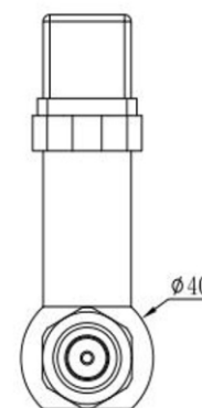
Hirschmann Connector Side View
