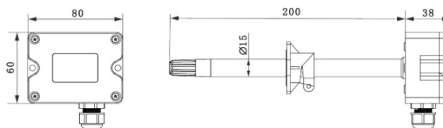
LFH10A2 Duct type
