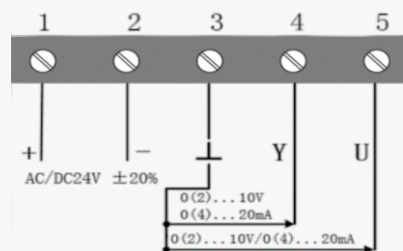
Volt0(0)...10V input resistance≥200KΩ Current0(4)...20mA input resistance=500Ω
