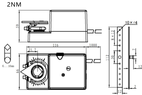
Dimension drawing: 4-6NM
