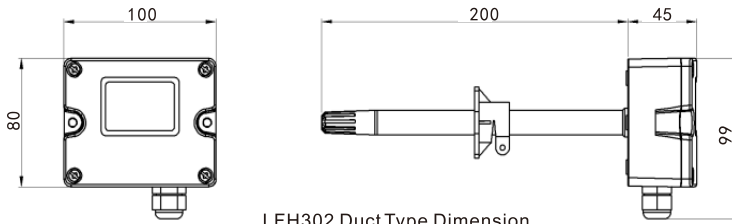
LFH302 Duct Type Dimension
