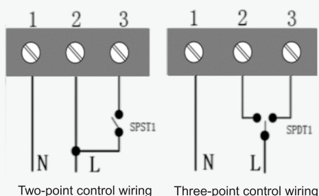
Switch output connection method, Working voltage: AC/DC 24V; AC100V...AC240V
