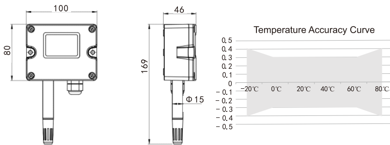
LFH301 Wall-mounted type dimension
