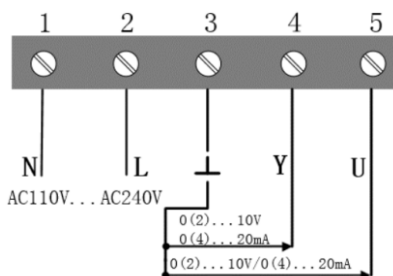
Volt0(0)...10V input resistance ≥ 200KΩ Current0(4) ... 20mA input resistance = 500Ω Analog wiring, supply voltage AC100V...AC240V
